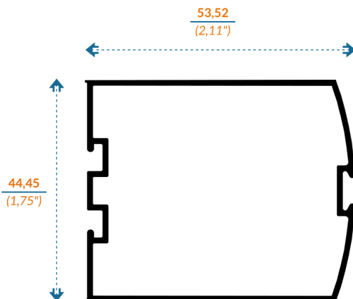
9204/2-5022 CERCO CHAPA
