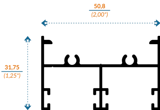
7518/21828 CHAMBRANA
