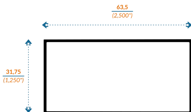
V11099 TUBO 2" 1/2 x 1" 1/4
