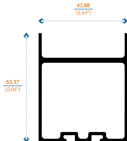
9207/15020 CABEZAL
