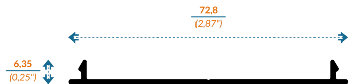
V7316 TAPA LISA
