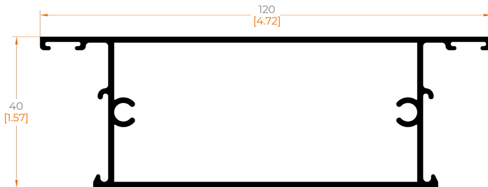
1422 ZOCLO CENTRAL
