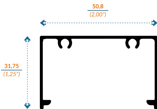
V8591 BOLSA LISA
