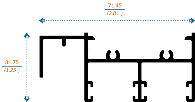
7819/16414 CHAMBRANA MOSQUITERO
