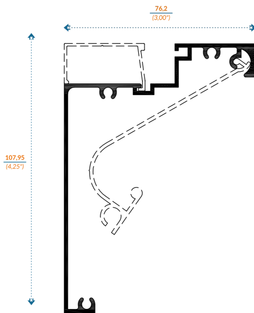
10465/6220 CABEZAL
