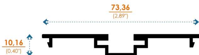
10237 TAPA CHAMBRANA
