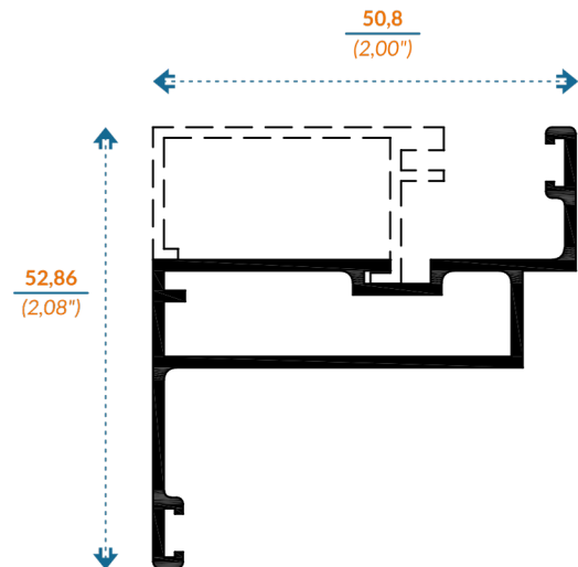
8936/16213 MARCO
