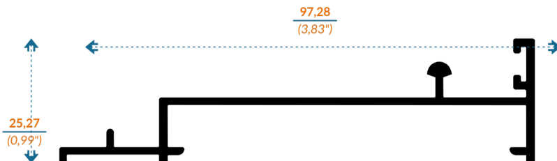
9272/2-7008 RIEL MOSQUITERO
