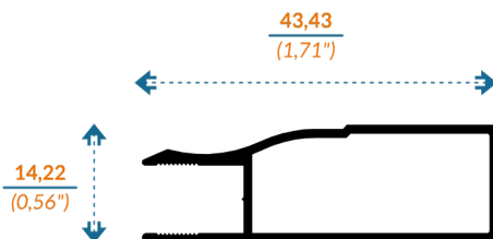
9756/22140 MARCO SEMI LUJO
